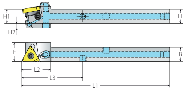
ALCS Type (with Anvil) & NLCS Type (without Anvil)
