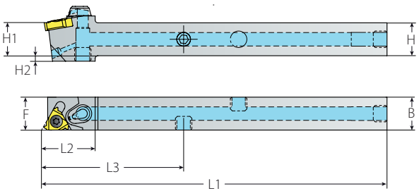
NLCS Type (without Anvil)
